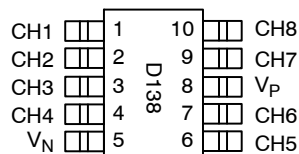
Pin Schematic
